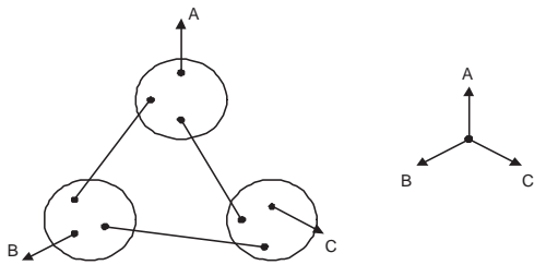
FIG. 9: A graph made of three communities. The three sources lie in different communities. The angle between any two of the weight vectors A , B and C is 120 degree.
